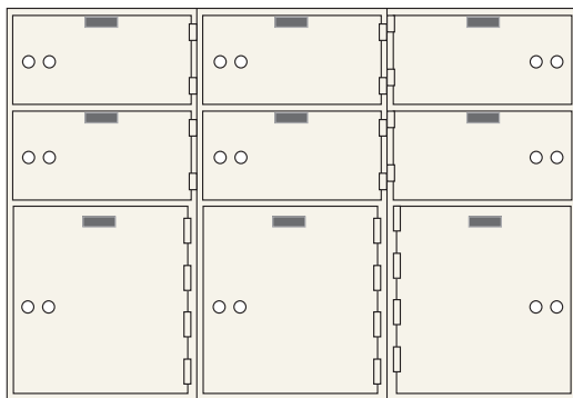
AX-9 (Wt. 195 lbs.) 6 openings ea. 5" x 10" 3 openings ea. 10" x 10"
